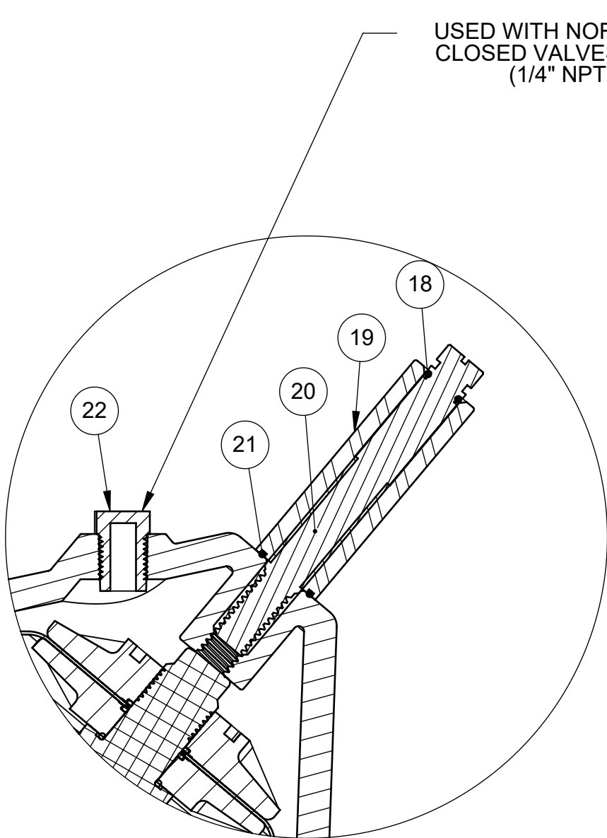
1070181 (K526-X210-14000) LIMIT STOP
