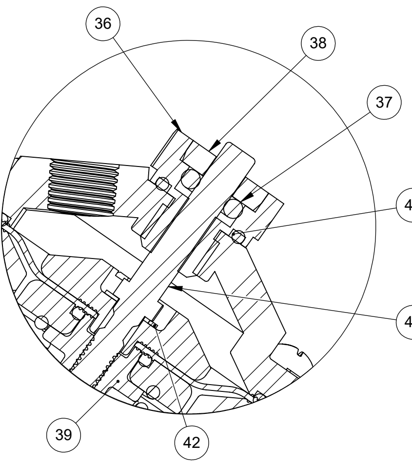
1071079 (K520-X221-14000) POSITION INDICATOR
