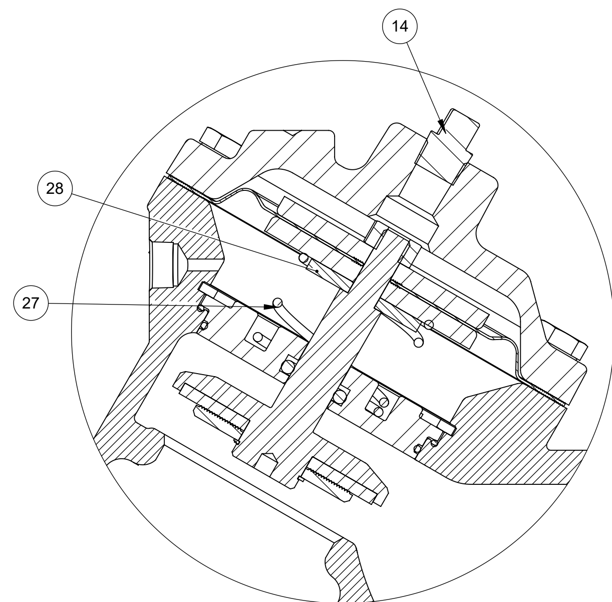
SPRING ASSIST OPEN MODEL:V46F-3201-03000 (FLANGED) MODEL:V46F-0201-03000 (THREADED)
