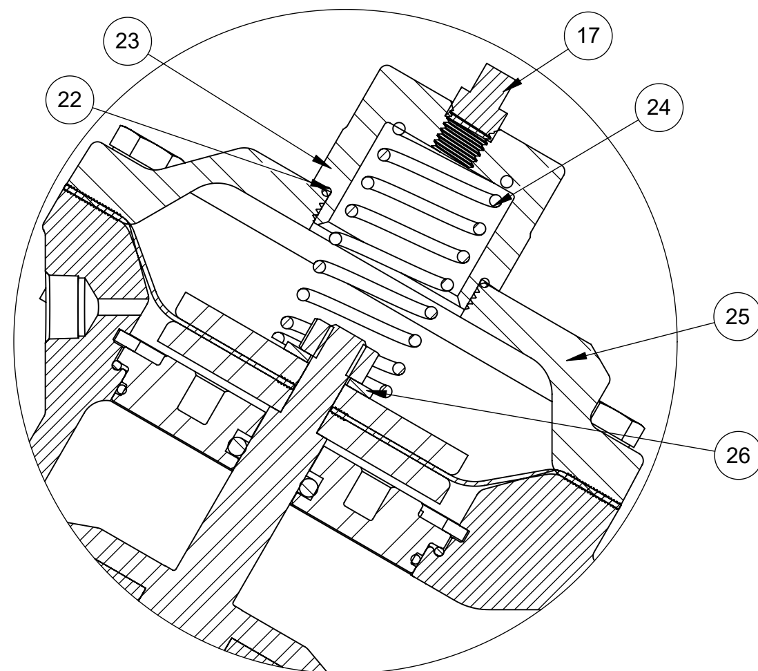
SPRING ASSIST CLOSED MODEL:V46F-3202-03000 (FLANGED) MODEL:V46F-0202-03000 (THREADED)
