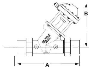
Male Socket Weld End Connectors
