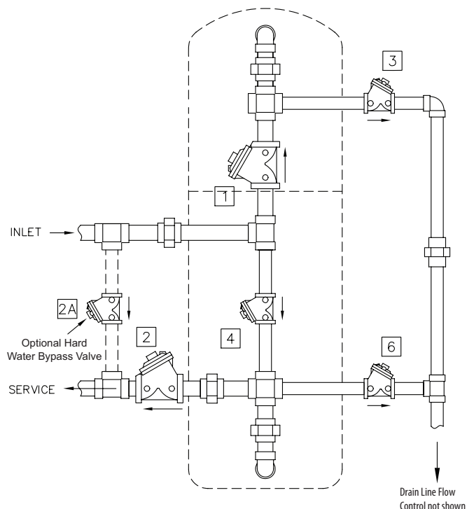
4 POSITION FILTER
